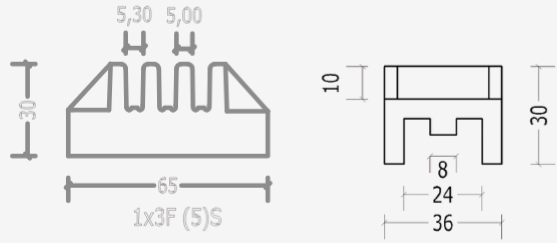
1x3F(5)S Busbar Support / Order Code: 30010102
