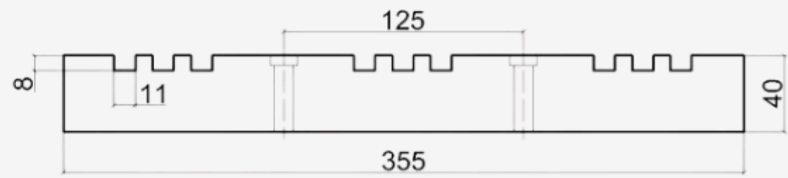
DBT-3x3FB (125 mm.) Busbar Support Order Code: 20030101
