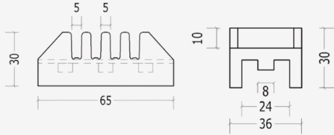
1x4F(5)S Busbar Support / Order Code: 35010102
