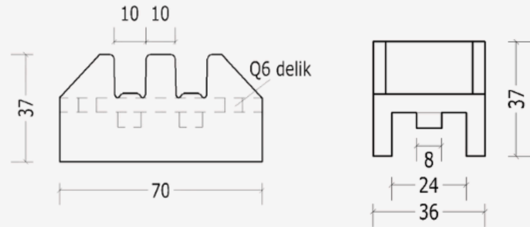
1x2F(10)S Busbar Support / Order Code: 35020102
