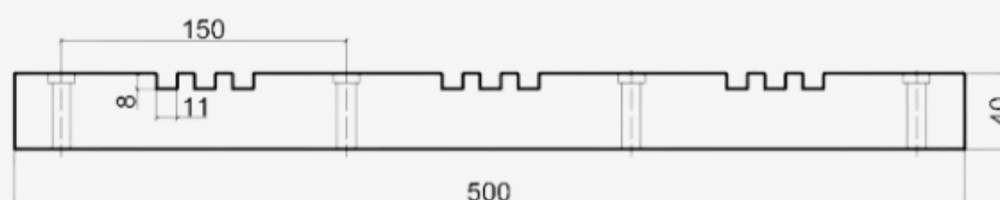
DBT-3x3FS (150 mm.) Busbar Support Order Code: 20040102
