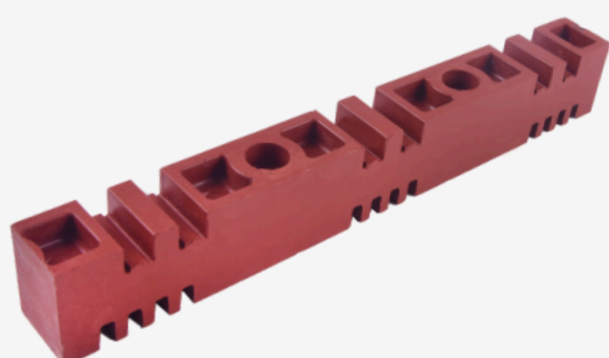
DBT-3x2FB/M Multi Series Busbar Support / Order Code: 20060101
