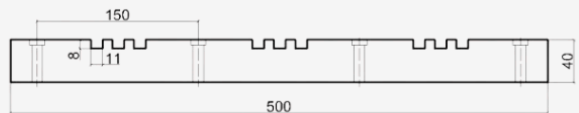
DBT-3x3FB (125 mm.) Busbar Support Order Code: 20030101
