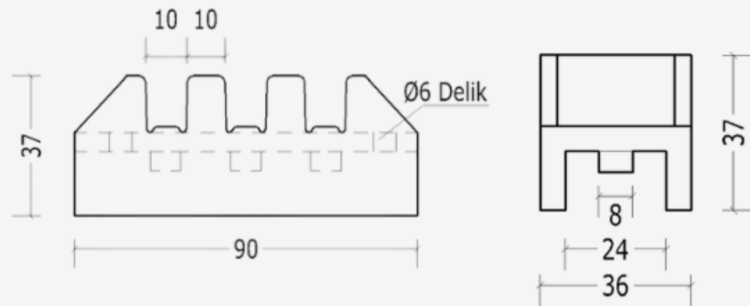
1x3F(10)S Busbar Support / Order Code: 35030102
